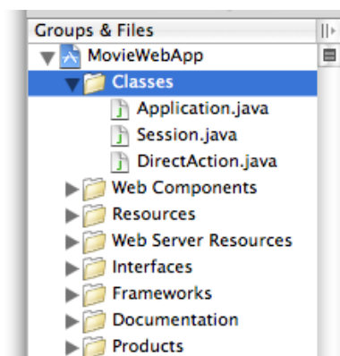
Figure 5 Classes group
