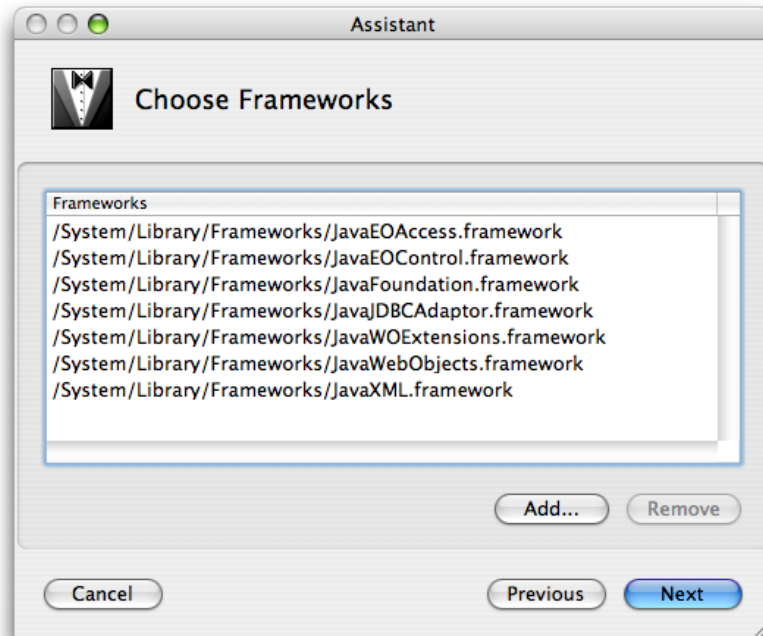
Figure 4 Choosing frameworks
