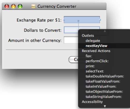
Figure 4-11 Connecting nextKeyView outlets in Interface Builder
