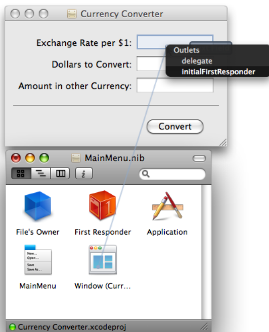
Figure 4-12 Setting the initialFirstResponder outlet in Interface Builder
