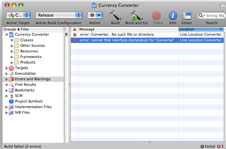
Figure 6-1 Identifying build errors
