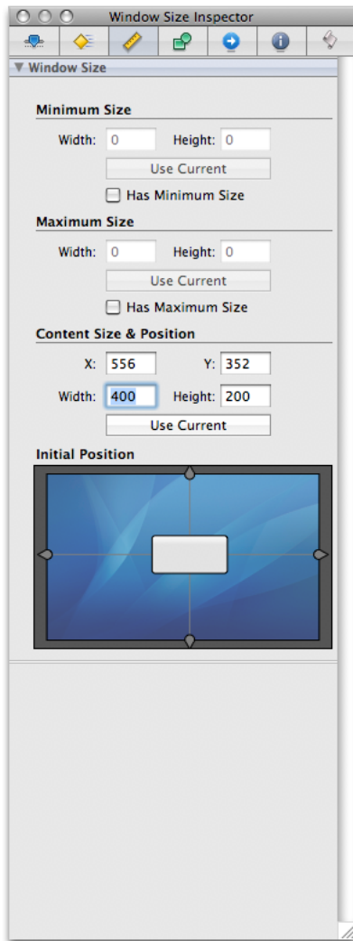
Figure 4-2 Resizing a window with the inspector
